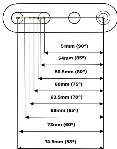
Outer pin hole
